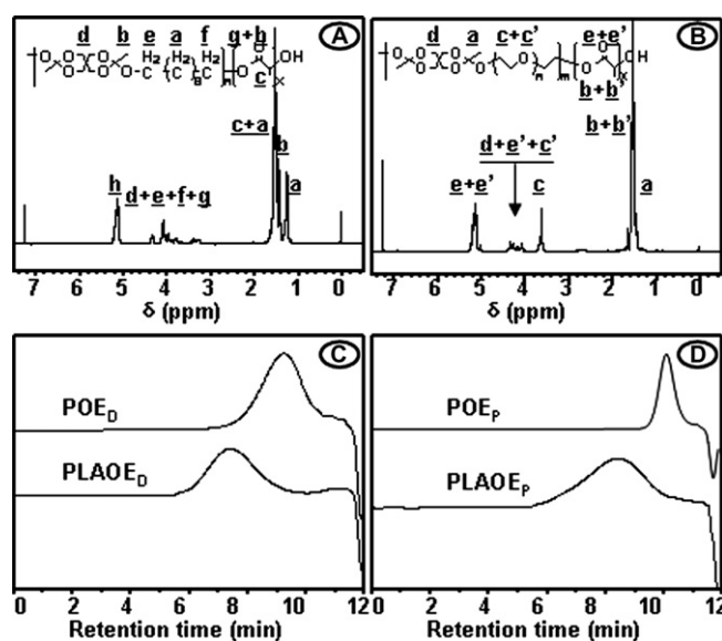
Fig. 2. ^1\text{H} NMR spectra of PLAOD (A) and PLAOP (B); GPC elution profiles of POED and PLAOD (C), POEP and PLAOP (D).
