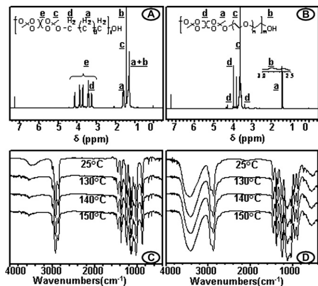
Fig. 1. ^1\text{H} NMR spectra of POED (A) and POEP (B); FTIR spectra of POED (C) and POEP (D) after incubation for 2 h under elevated temperatures.
